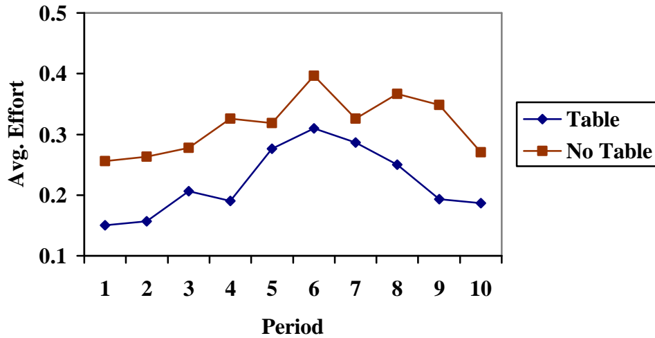
Figure 3 Avg. Effort over Time
