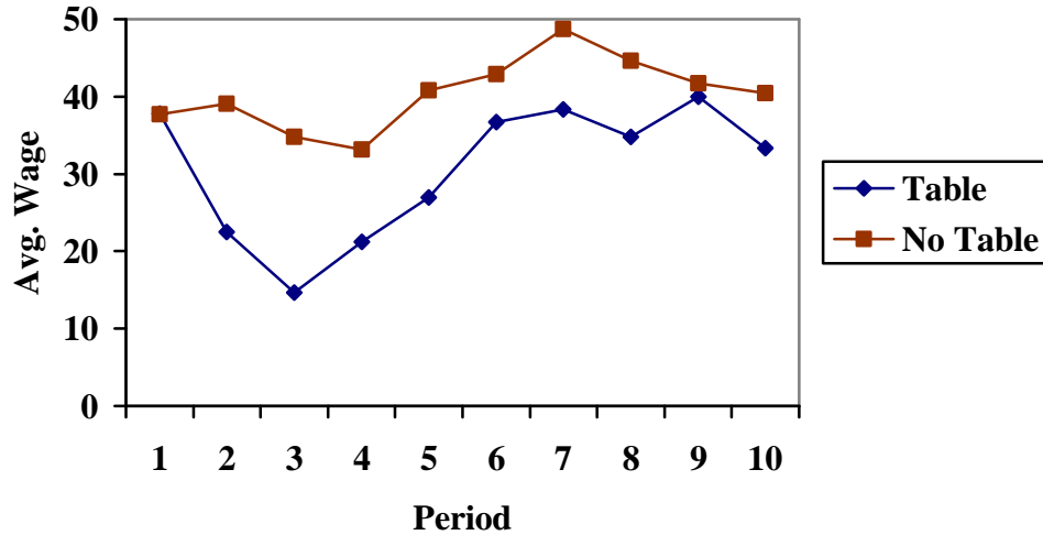
Figure 4 Avg. Wage over Time
